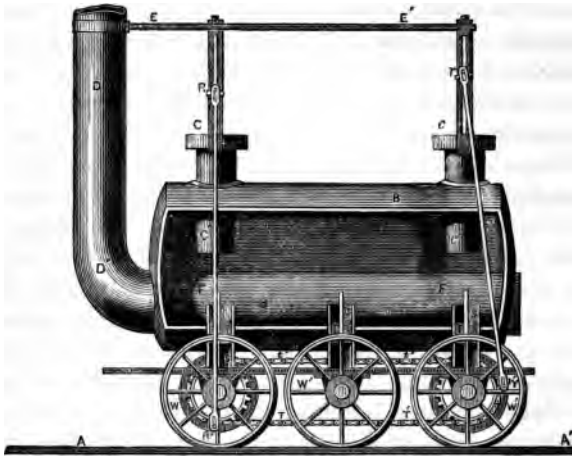
FIG. 51.—Stephenson's Locomotive of 1815. Section.
